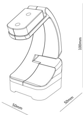
Security Display stand MAX830_V2
